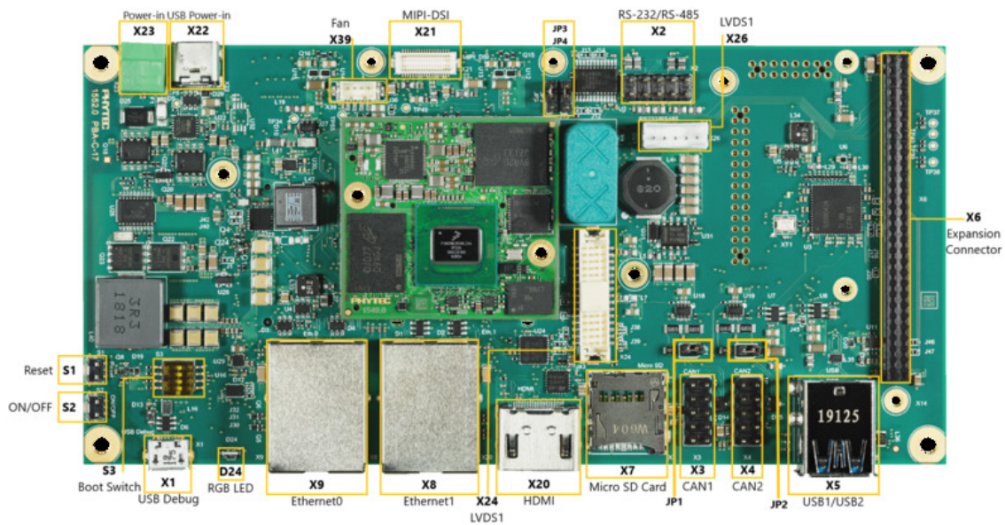
图 1: Libra Components (top)
