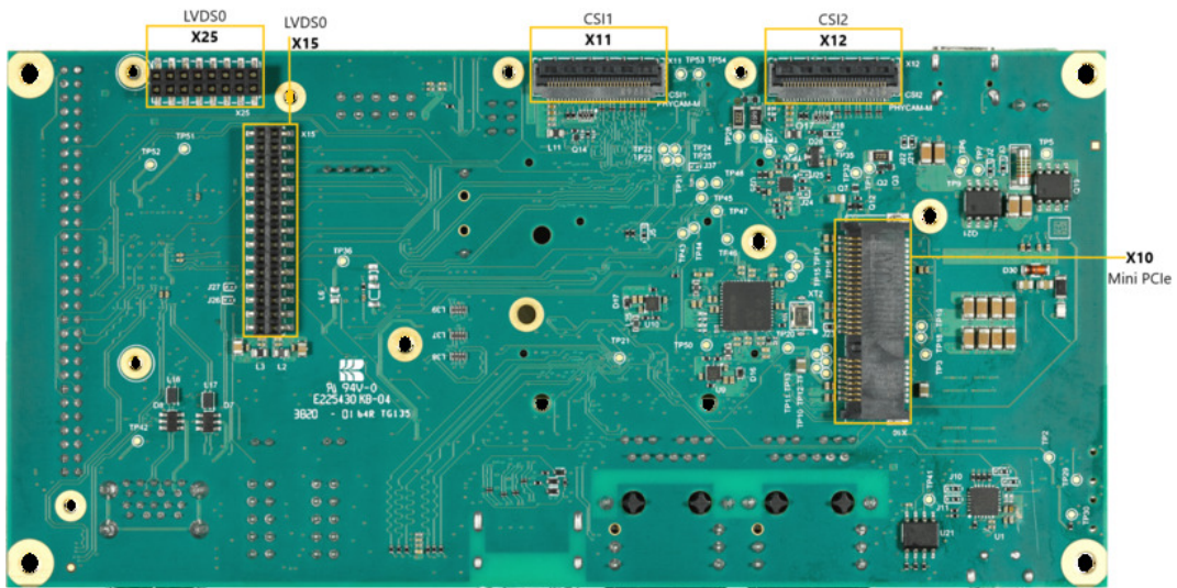
图 2: Libra Components (bottom)
